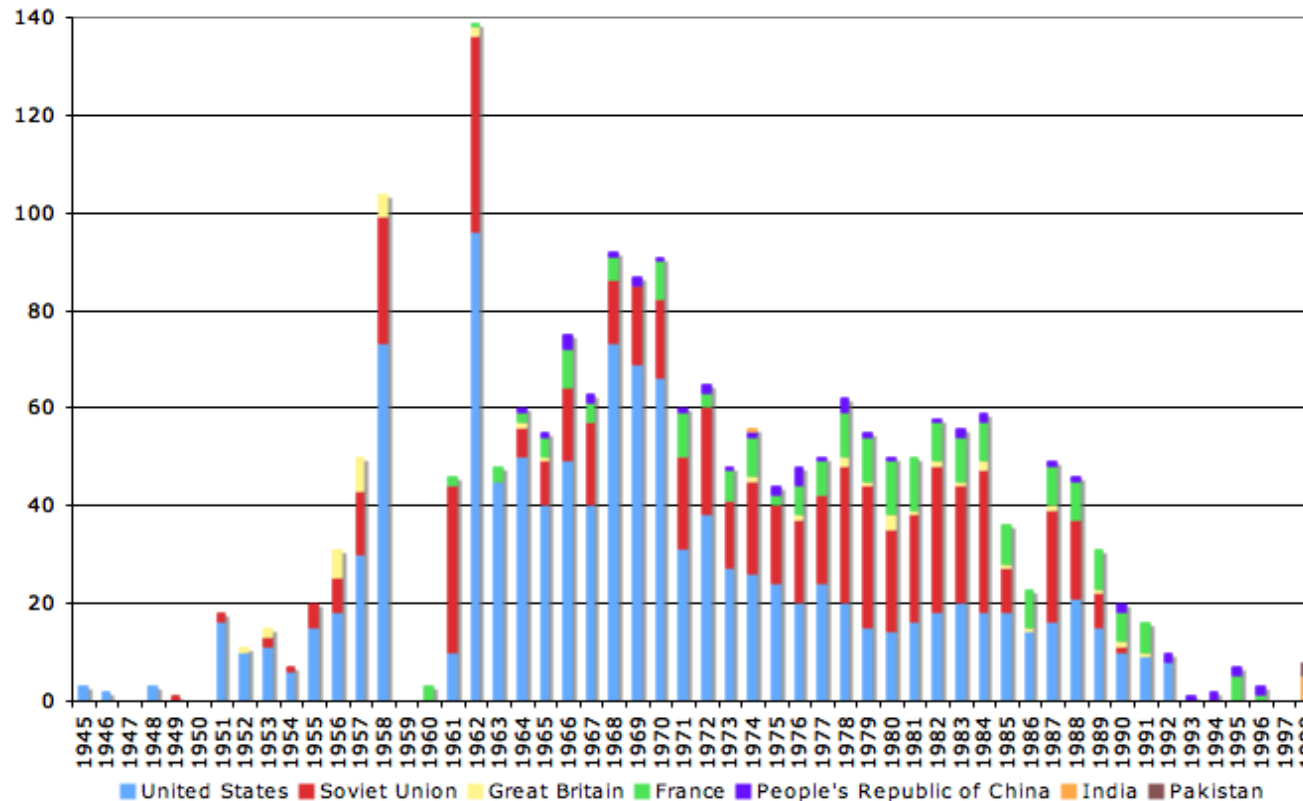
Worldwide nuclear testing, 1945-1998
